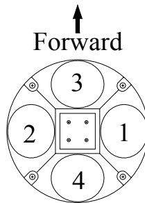
Figure 18. View facing an ADCP transducer. The layout is the same for both convex and concave transducers (see Figure 26).
